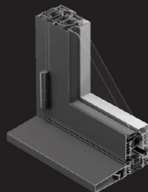
CONTEMPORARY SBF100/SBF301 [Clip-on Cill SA033]
