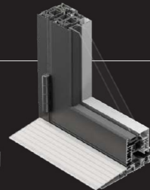
CONTEMPORARY SBF100/SBF301 [Ramped Low Threshold SBF700]
