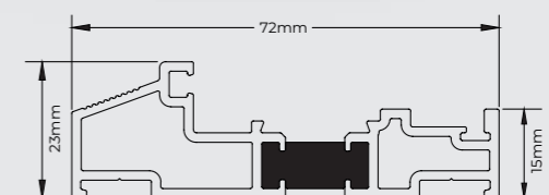
SP713 49mm COMPOSITE DOOR LOW THRESHOLD
