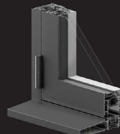
INTEGRAL CILL SBF400
