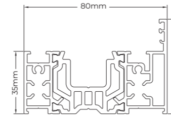
SBF100 - OUTER FRAME
