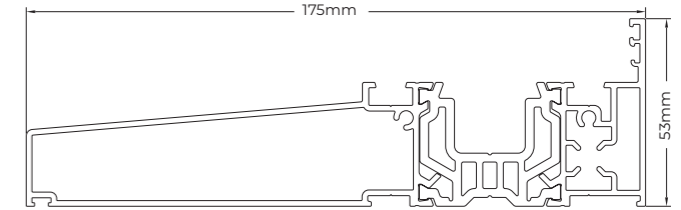
SBF400 - INTEGRAL CILL
